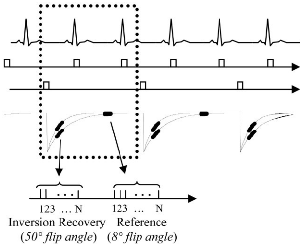
FIG. 1. Pulse sequence diagram for single-shot inversion recovery true-FISP with acquisition of IR and reference images for PSIR image reconstruction. Data for IR and reference images are collected alternately every other heartbeat.
